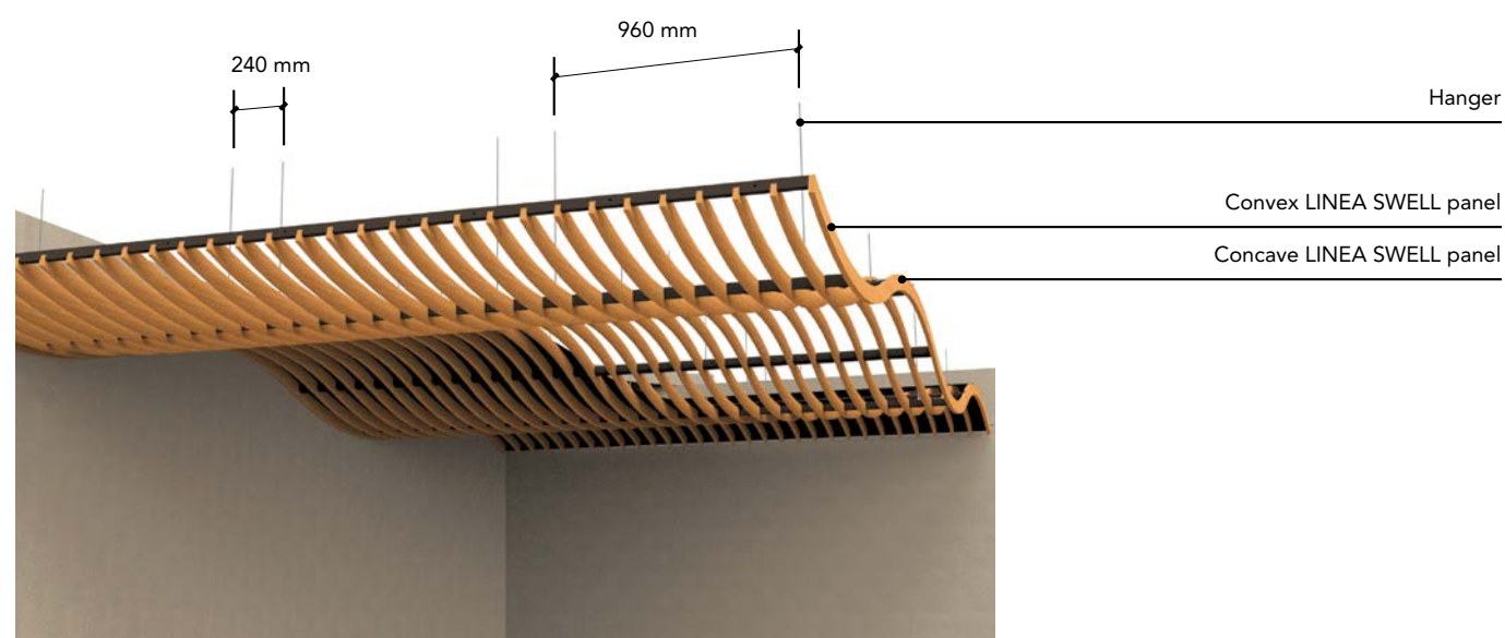
Bottom view
