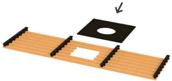
Step 4: Insert the particle plate on the panel
