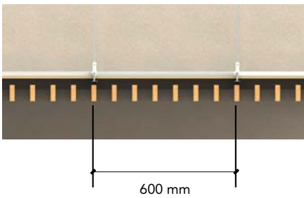
Transverse view
