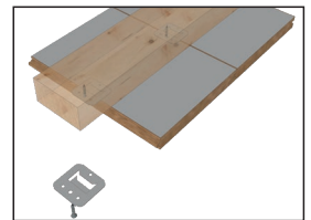
SC-System – with screw clips on wooden battens or metal substructure
