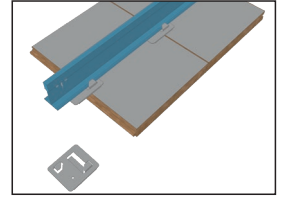
T-System – with turning clips on T-profile
