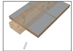
W-System – with staple machine on wooden battens
